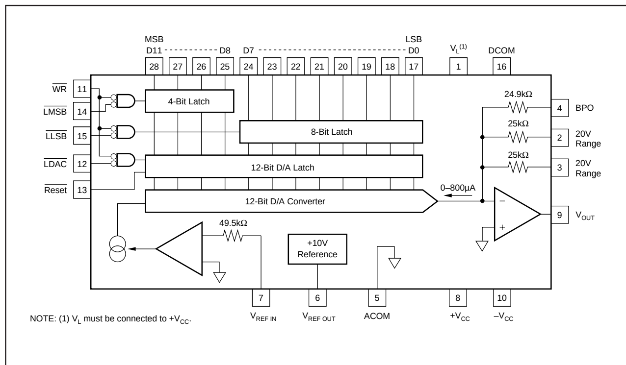
FIGURE 1. DAC813 Block Diagram.
